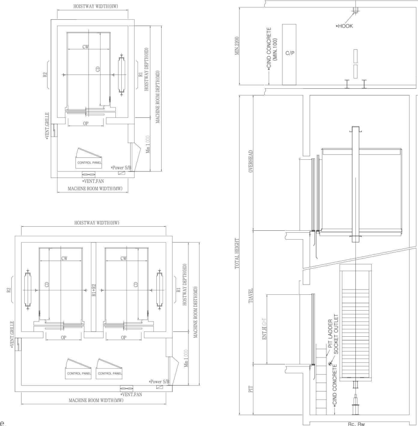
HOISTWAY SECTION
