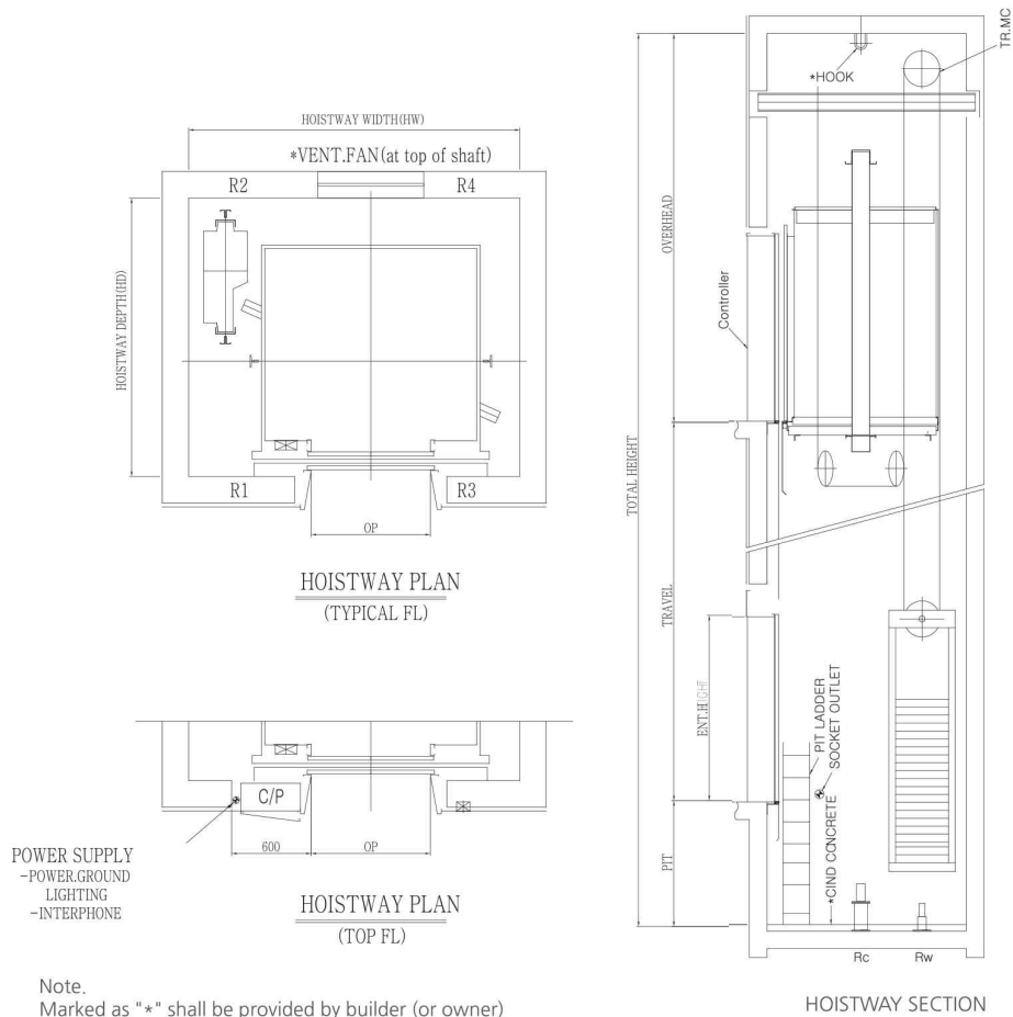
HOISTWAY SECTION
